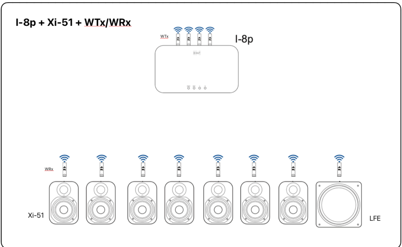
圖九：i-8p + WTx/WRx + Xi-51x7 + Xi-81
