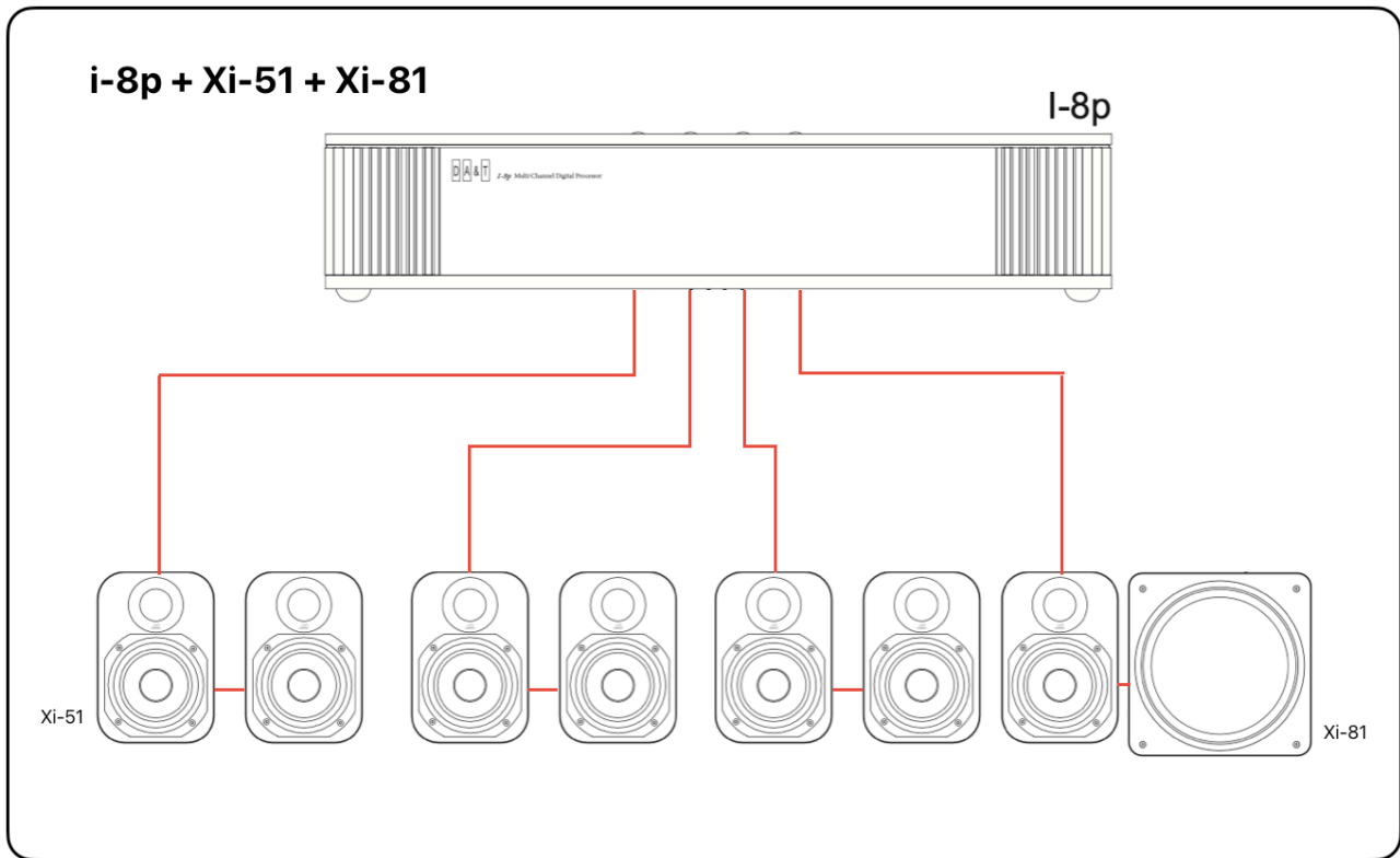
圖七：i-8p + Xi51x7 + Xi-81
