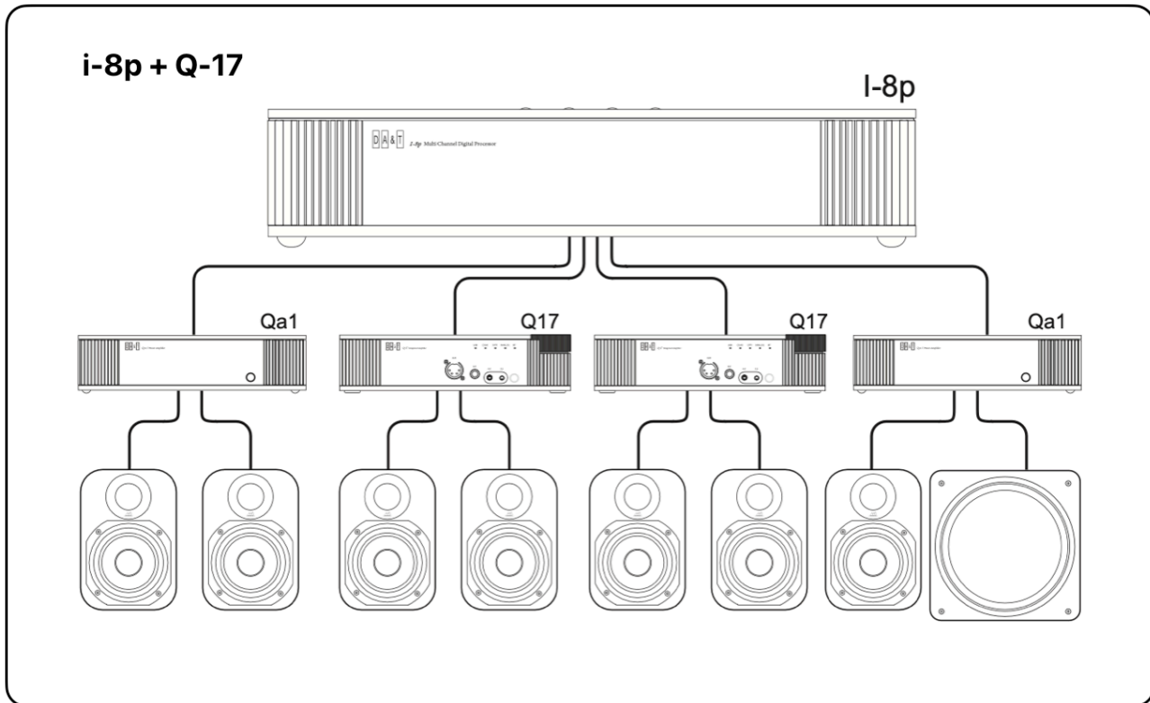
圖五：i-8p + Q-17x2 + Qa1x2
